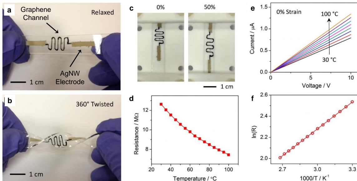
Figure 1.4. Stretchable graphene thermistors and characterization. (a, b) Images of the stretchable graphene thermistors at relaxed and twisted states. (c) Images of the stretchable graphene thermistor at 0 and 50% strains. (d) Resistance variation with temperature showing a nonlinear relationship. (e) IV curves of the thermistor at 0% strain in the temperature range of 30 to 100 °C. (f) Dependence of \ln(R) on 1000/T showing a linear relationship. Reproduced with permission [21]. Copyright 2015, American Chemical Society.
